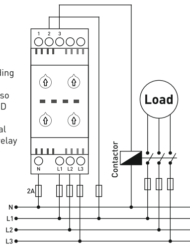
Connection Diagram for P1-PAV
