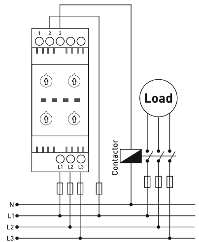
Connection Diagram for P1D-PAV
